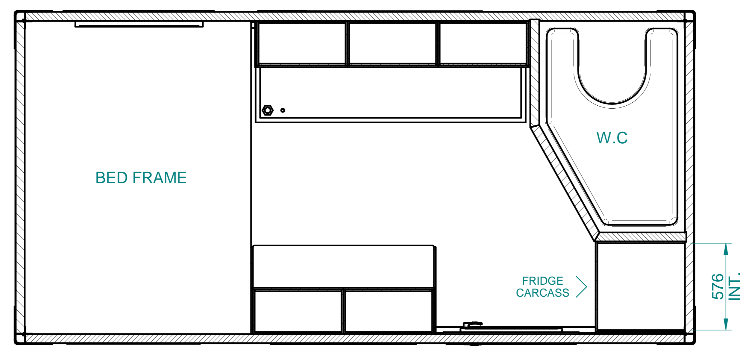
SECTION C-C
