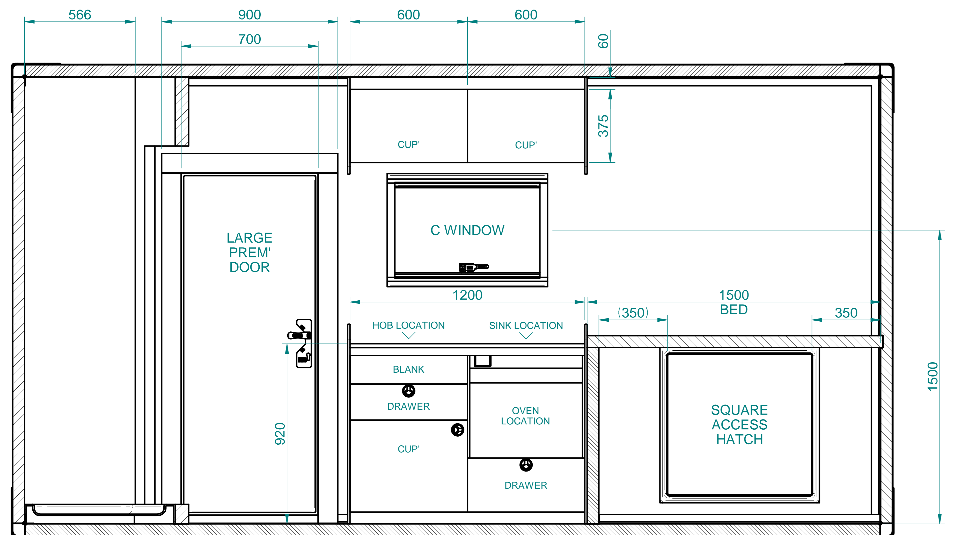
SECTION B-B 1:10
